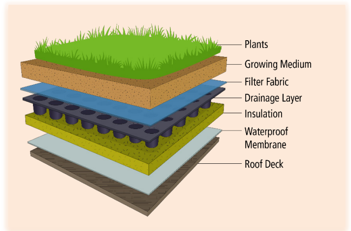
Green roof cross section showing typical material layers. Based on USEPA's diagram of The Common Green Roof Layers
